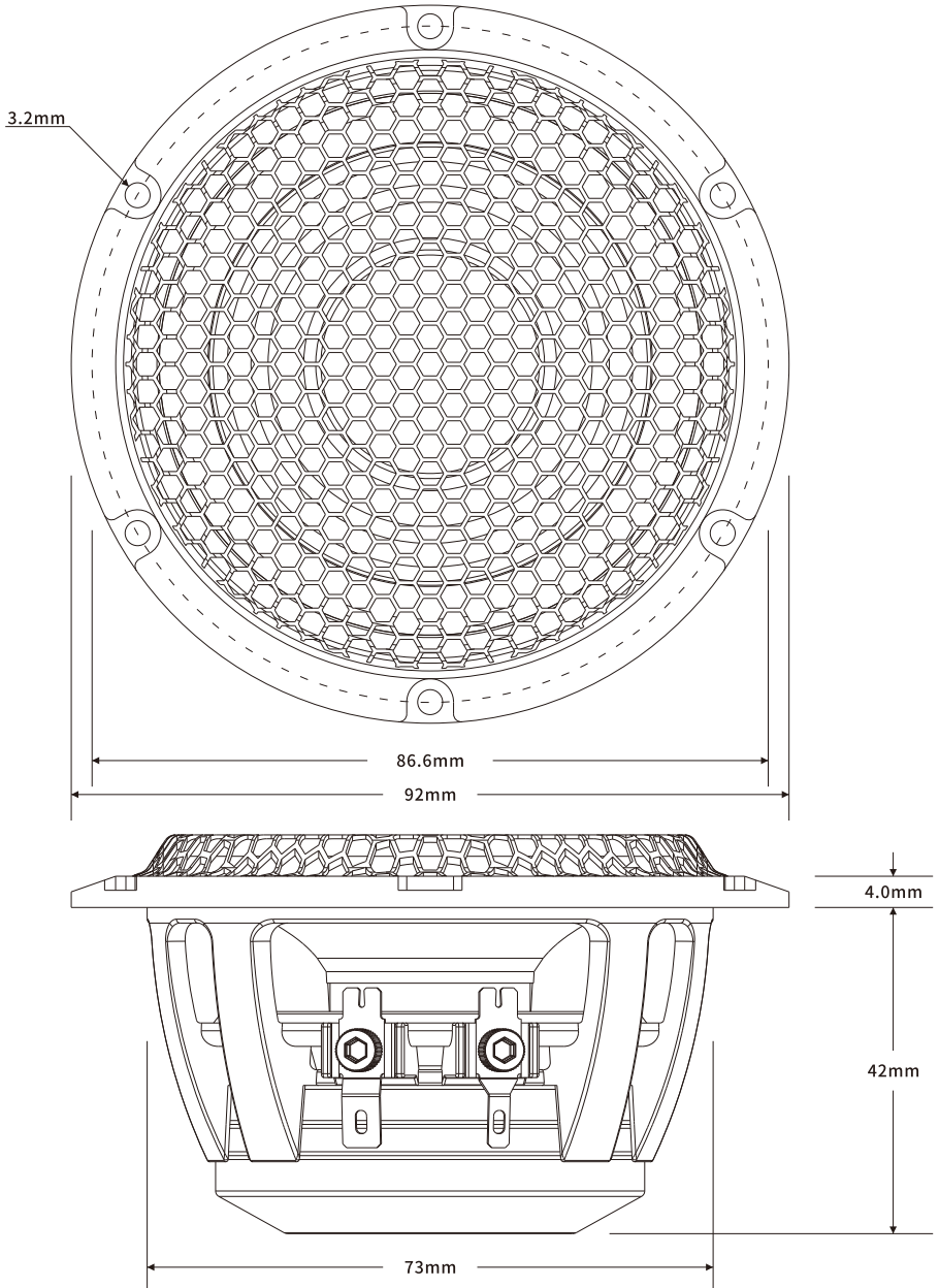
Speaker Dimension Drawing
